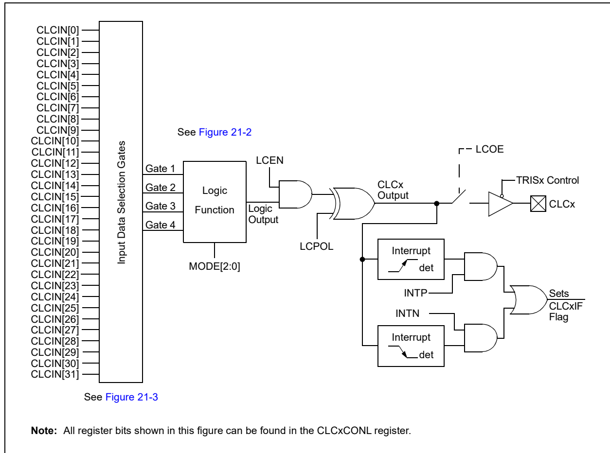
FIGURE 21-1: CLCx MODULE
